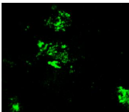
IF: Species protein in neutrophil extracellular traps (NETs) . Staining of azurocidin with antibody Z6718.
